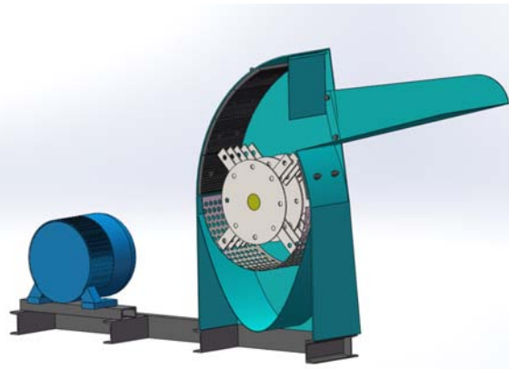
Multi functional hammer mill inner structure
